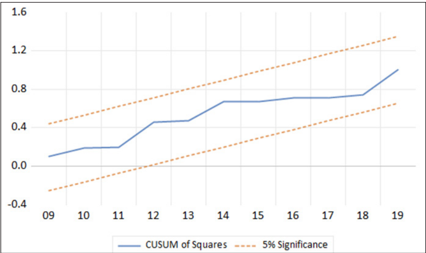
Figure 6. Plot of CUMSUM of Squares Note: The straight lines represent critical bounds at a 5% significance level
